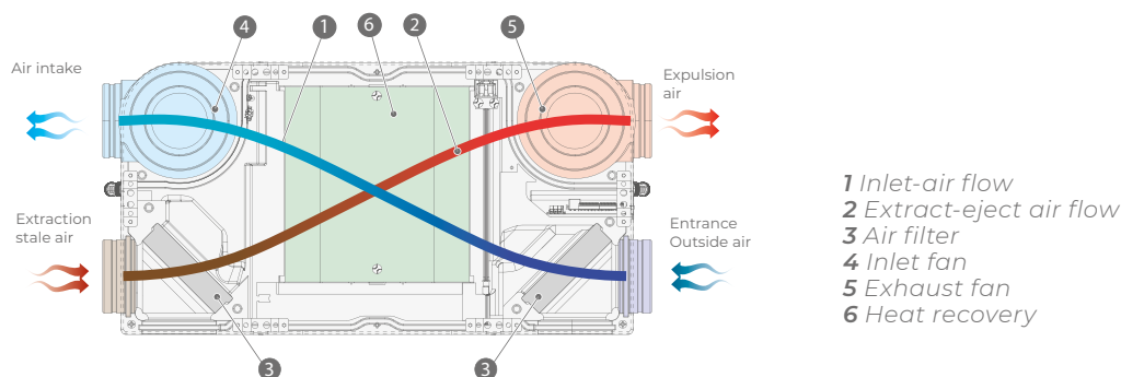
Operating principle of a dual-flow MVHR machine
