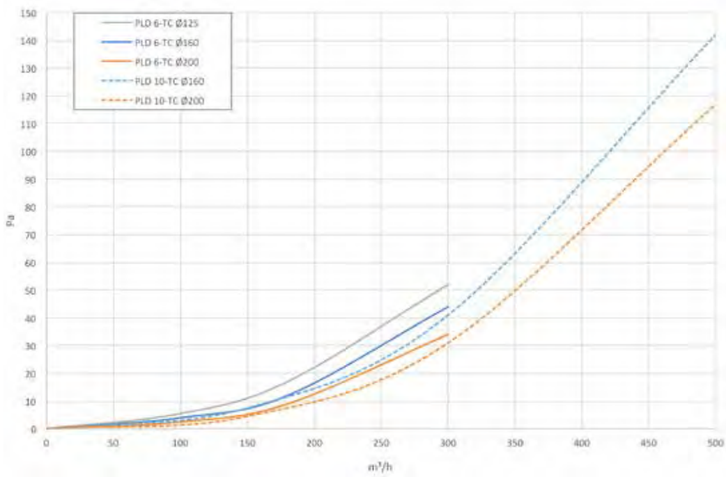
Plenum PLD-U - Stale air extraction
