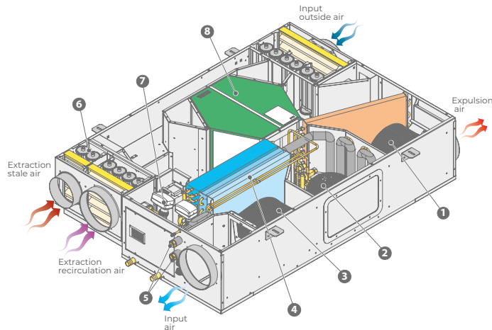
Operating principle of an air handling unit
